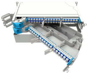
MFPS Fiber Optic Panel, 19inch, 2RU,72 fibers/HU, splice/patch, SMOUV /left, 144 LC/UPC, grade B
